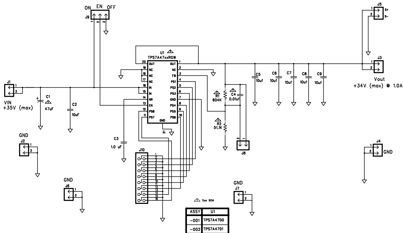
Figure 6. TPS7A47xxEVM-094 Schematic
