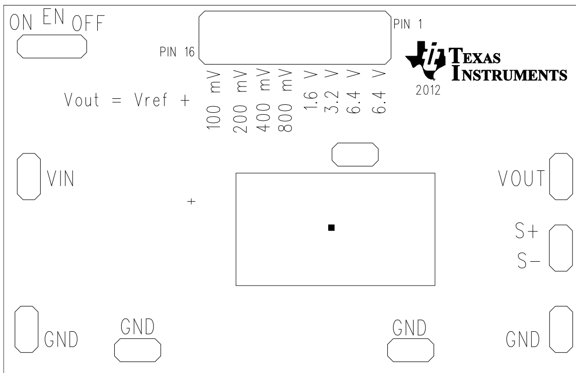
Figure 3. Assembly Layer
